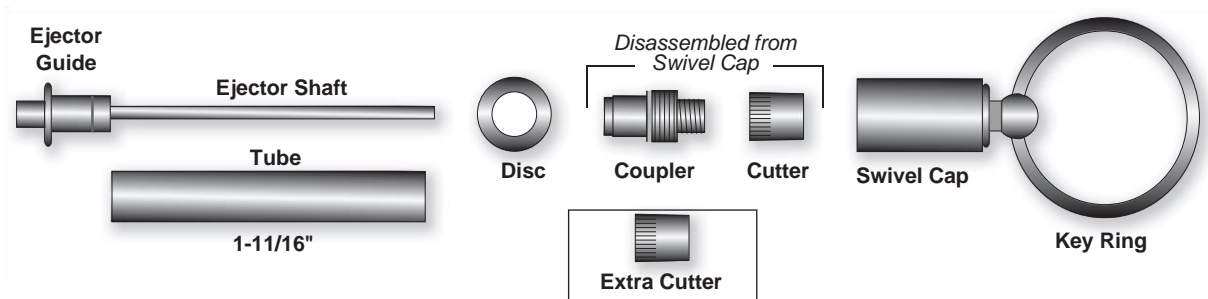
Diagram A - Parts and Assembly
