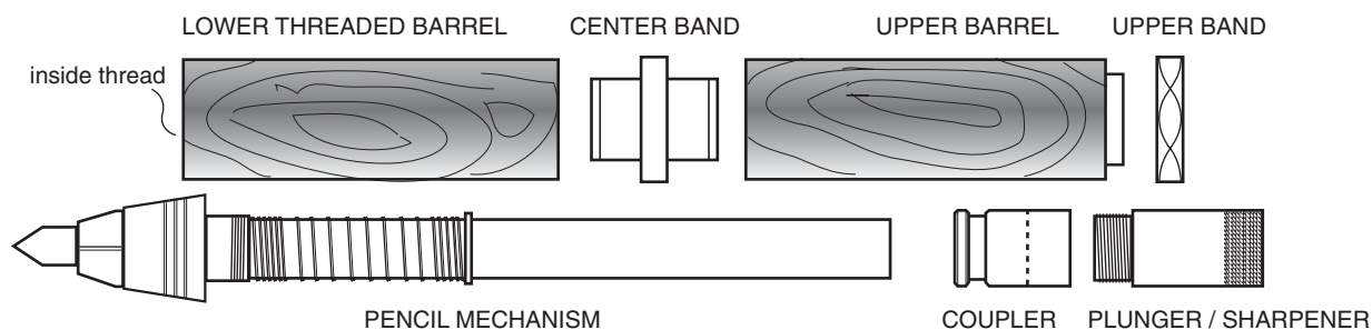
Diagram C- Assembly
