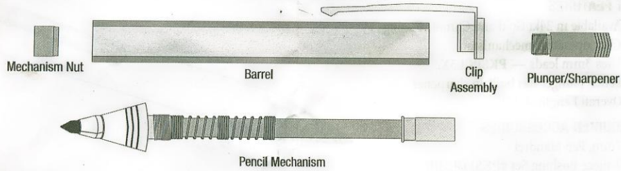
DIAGRAM C • Assembly
